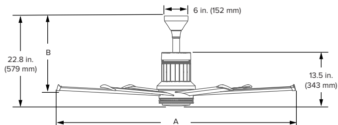
Pictured with 6 in. (152 mm) extension tube and light kit
