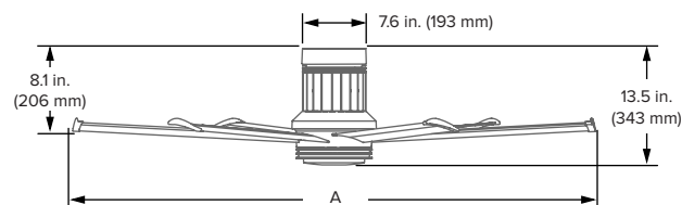
Pictured with direct mount and light kit
